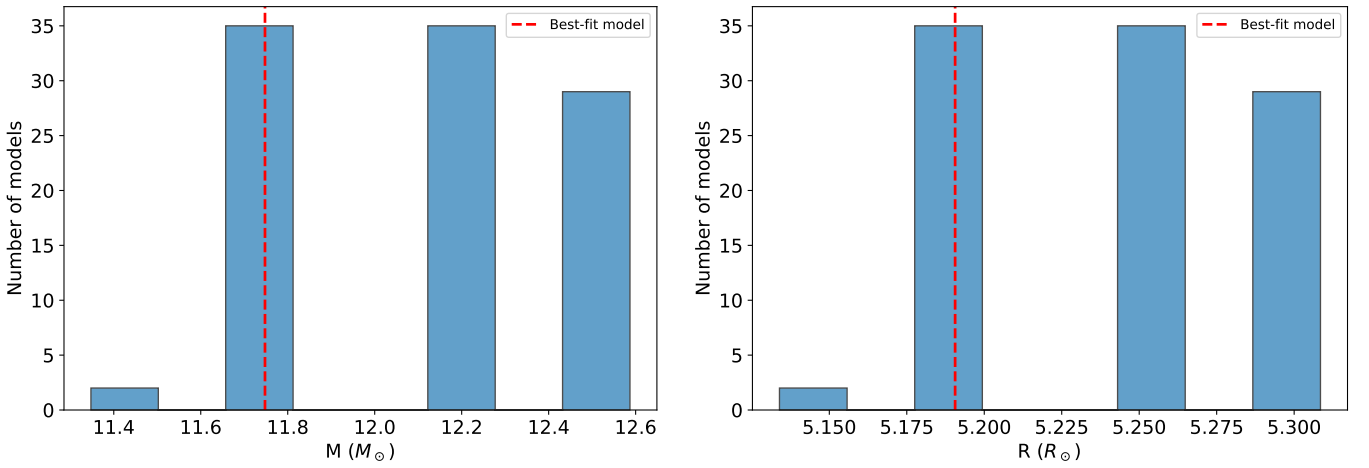
Fig. A.4: Example plots of the unweighted distributions of the derived parameters. The distributions of mass (left panel) and radius (right panel) of HD 112485 are shown for the \chi^2 models compatible with the spectroscopic constraints. The gaps in the unweighted distributions reflect the discrete sampling of the stellar-model grid and the subsequent selection of only models satisfying the adopted constraints. They are therefore not interpreted as evidence for physically distinct populations.
